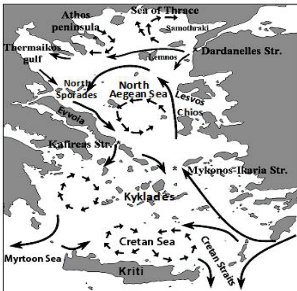
Fig. 2: Circulation of water masses in Aegean Sea (Nittis & Perivoliotis, 2002).
