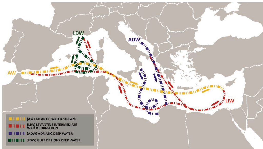
Fig. 1: Schematic diagram of the thermohaline circulation in the basin with the major conveyor belt systems indicated by dashed lines in different colour (redrawn after Pinardi & Masetti 2000).
